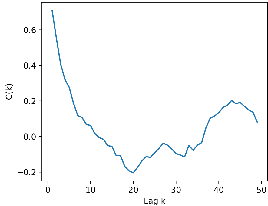
HOMO Autocorrelation
