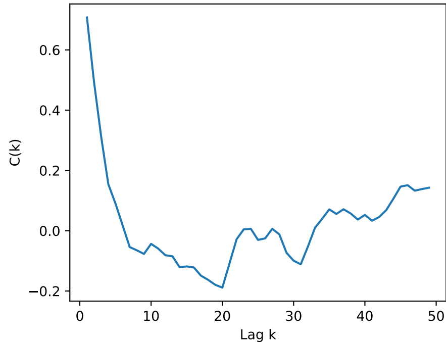
LUMO Autocorrelation
